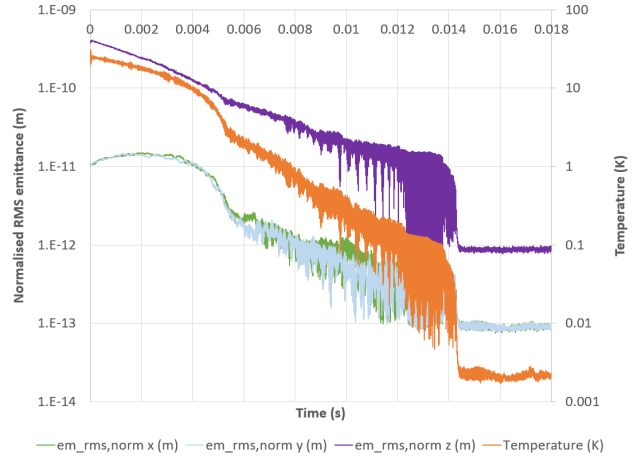
Figure 4: Laser Doppler cooling simulation with N = 500 ions.
