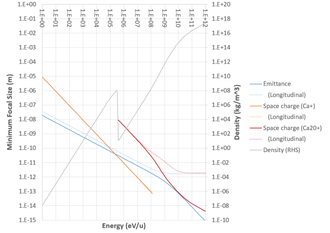
Figure 8: Focal size and density as a function of energy, with 20 times smaller initial emittance and twice the energy spread.
