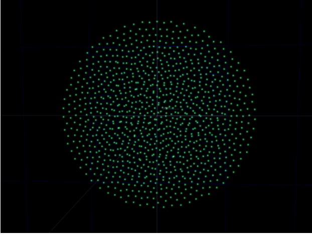
Figure 5: 2D Coulomb crystal that can be created by an anisotropic trap.
