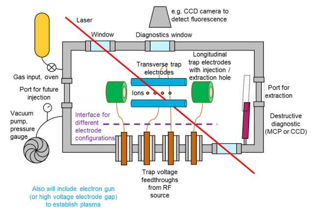
Figure 14: Schematic of ion trap system.
