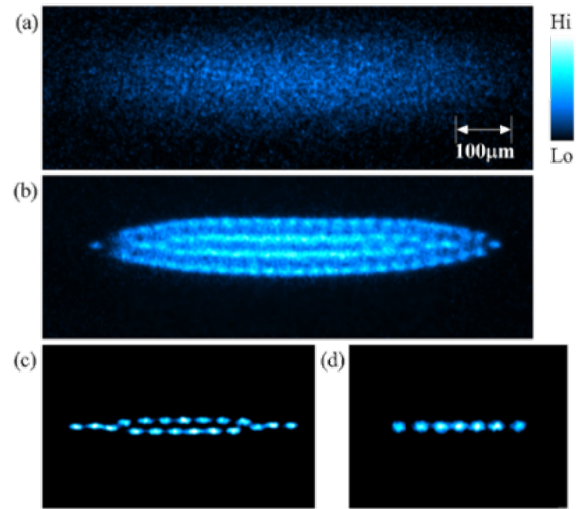
Figure 2: Fluorescence of a Coulomb crystal in the S-POD trap [3] at the University of Hiroshima.
