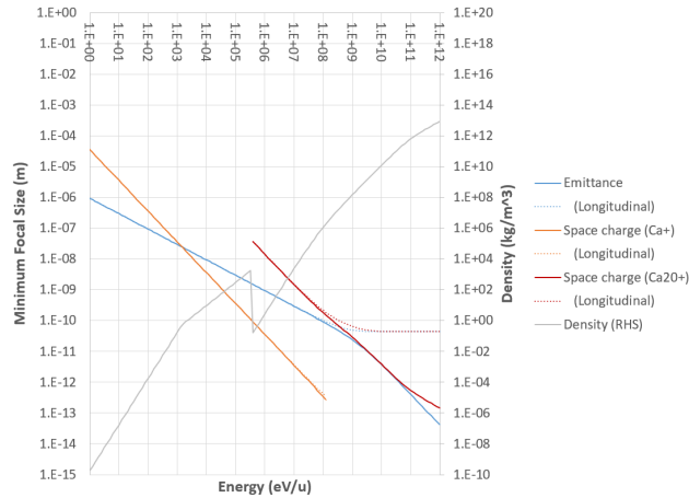
Figure 7: Focal size and density as a function of energy.
