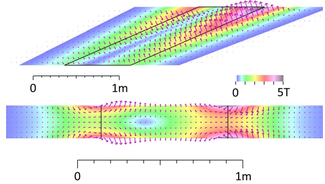
Figure 1: Cross-section of the 5 GeV ring magnet's field in ZY (top) and ZX (bottom) planes.
